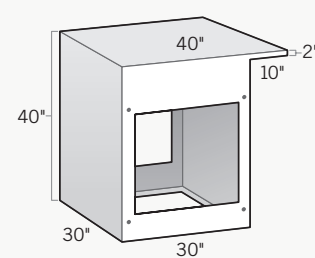
Bar-Height Cabinet with 10" Cantilever Backside 30"D × 30"L × 40"H
