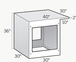
Cabinet with 10" Cantilever Backside 30"D × 30"L × 36"H
