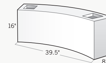
Curved Seating Wall (1/8 Circle) 8"D × 39.5"L × 16"H
